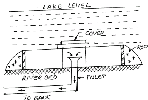
Fig 3.11 Lake Intake
