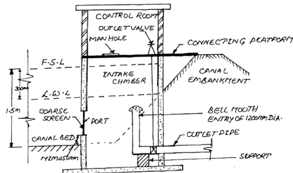
Fig. 3.14 Canal Intake
