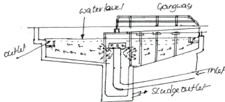
Fig 5.2 Sedimentation with Coagulation
