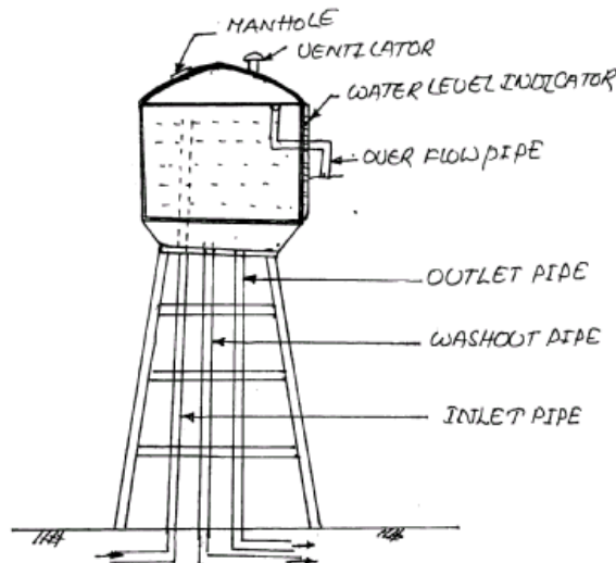
Fig 8.5. Overhead Tank
