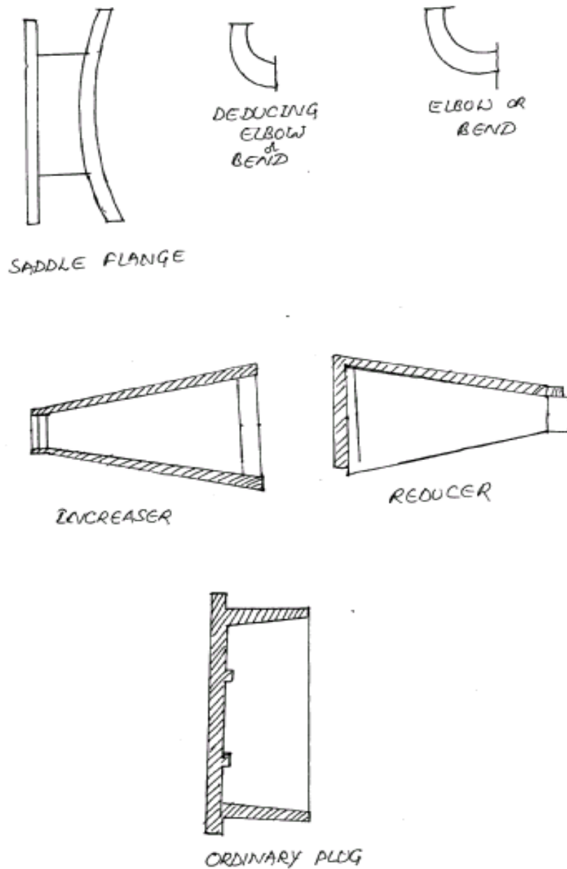
Fig 8.4 Pipe Fittings
