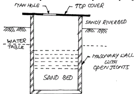
Fig 3.3 Infiltration Well
