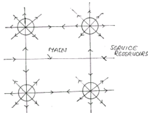
Fig. 6.4 Radial System
