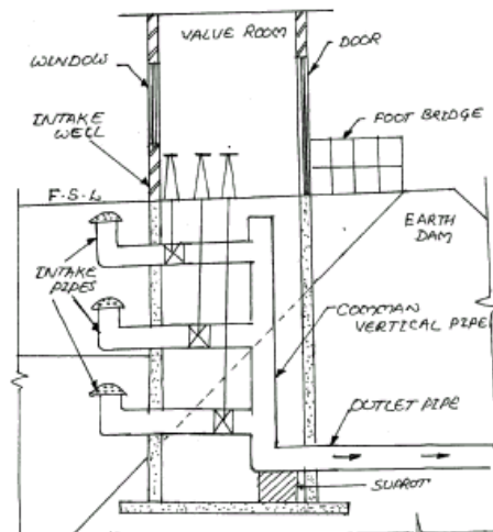
Fig. 3.13 Reservoir Intake
